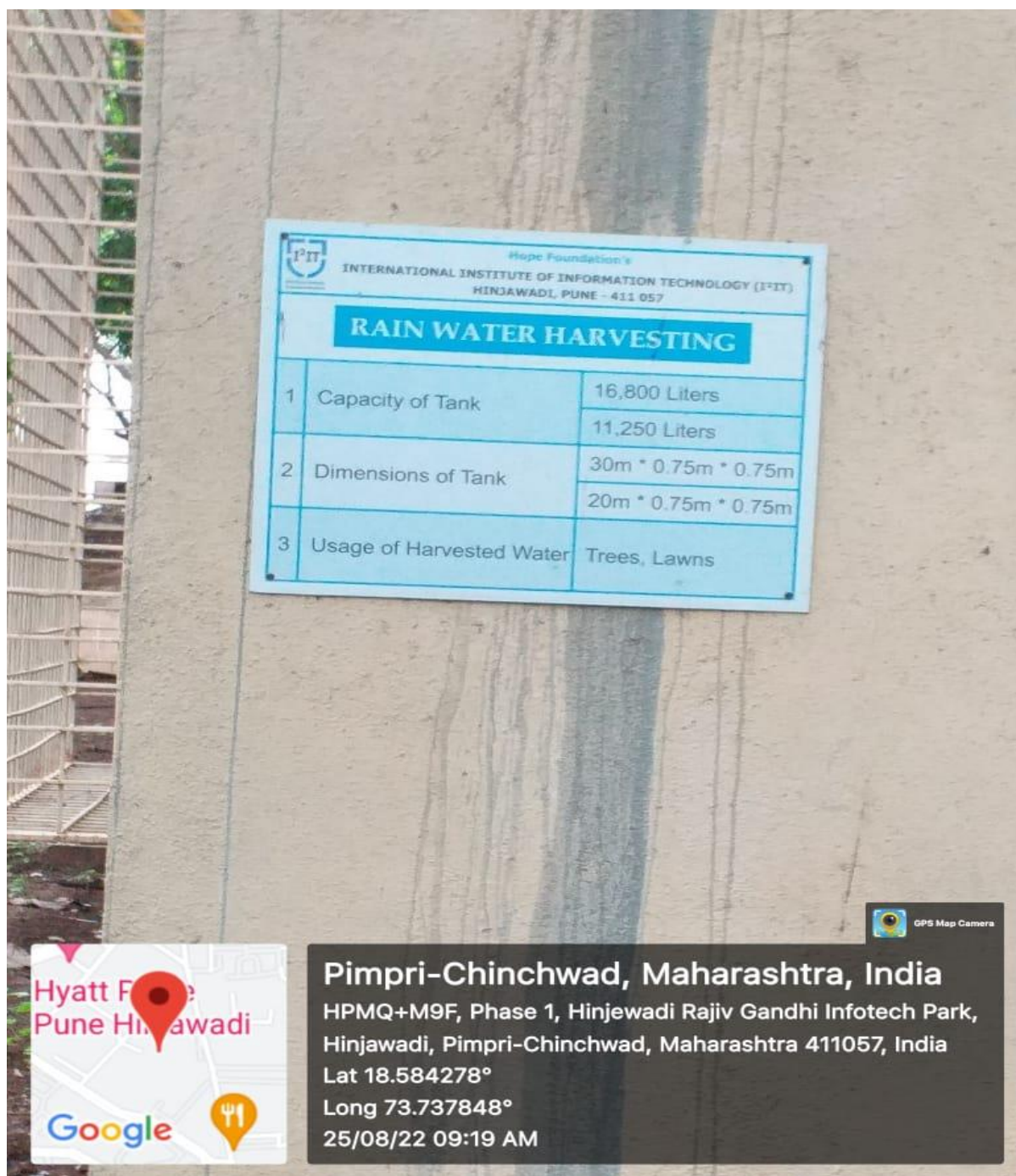
Rain water harvesting plant specifications
