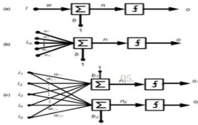
Fig 1: Neuron Models a) Neuron Model b) Multi-input Neuron Model c) Multi- input multi-neuron model
