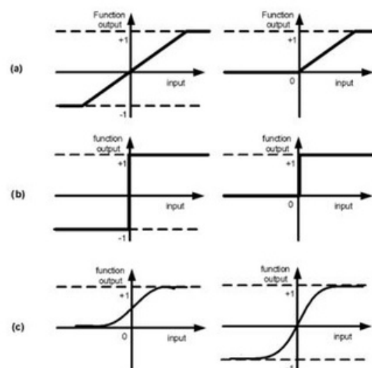
Fig 2:Neuron activation functions: a) linear bipolar (left) and unipolar (right) activation functions b) signum (left) and threshold (right) activation functions, c) sigmoidal or log-sigmoid (left) and hyperbolic or tan-sigmoid (right) activation function
